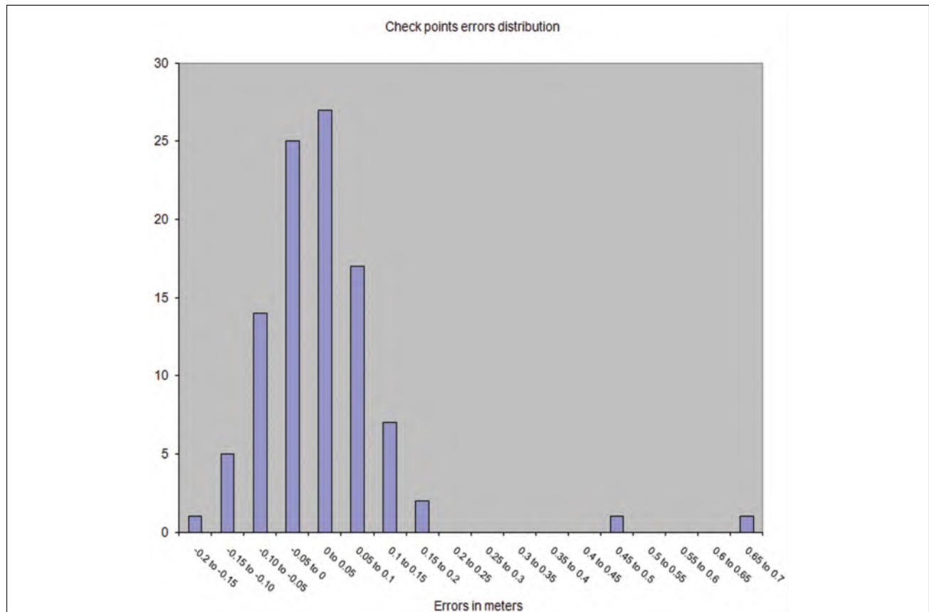
Plate D.1 Error Histogram of Typical Elevation Data Set, Showing Two Outliers in Vegetated Areas.
